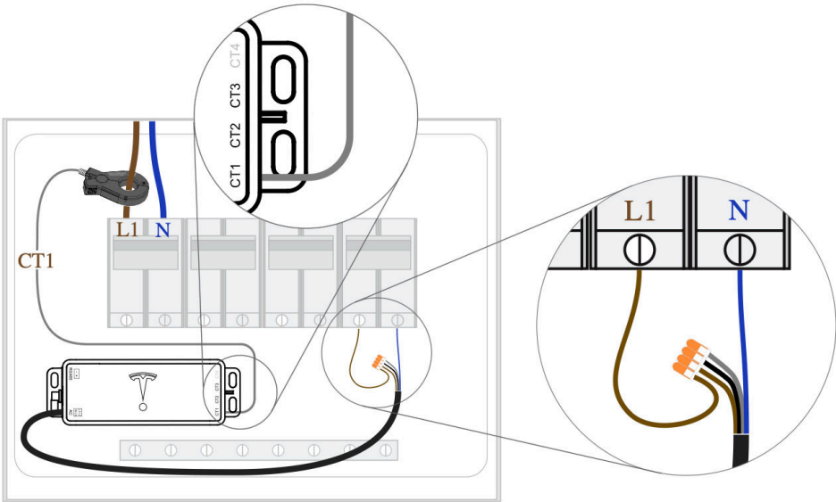
Figure 1. Configuration of remote meter inside panel - Single-phase
